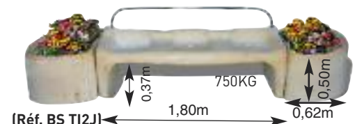
BANC STANDING
